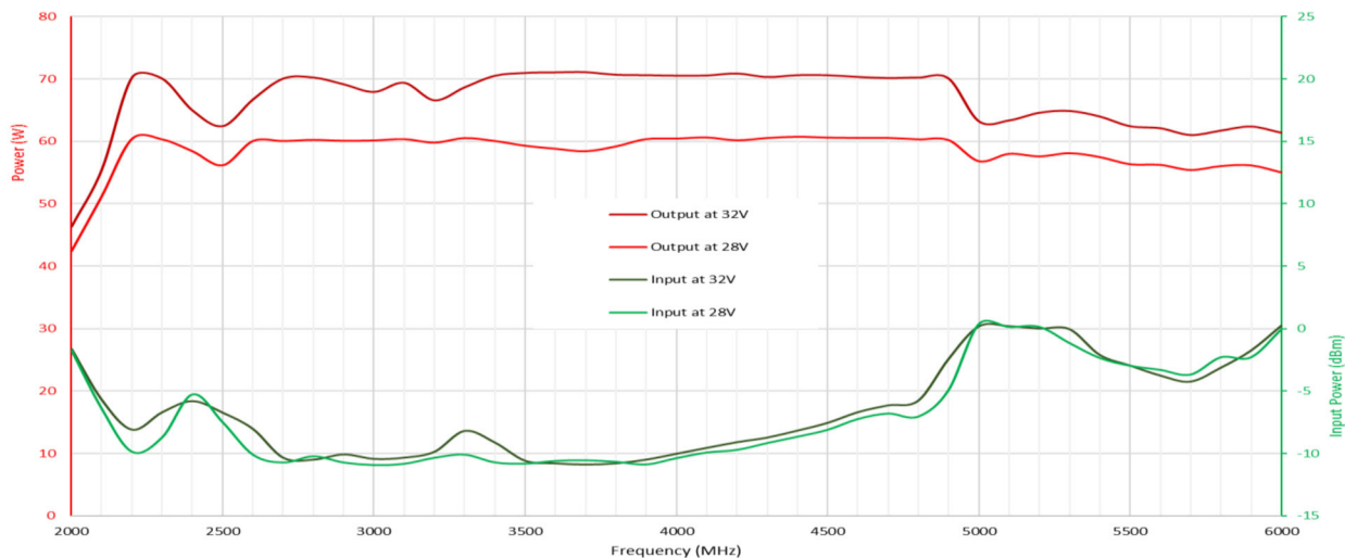
VM3F Psat Power / Input Drive
